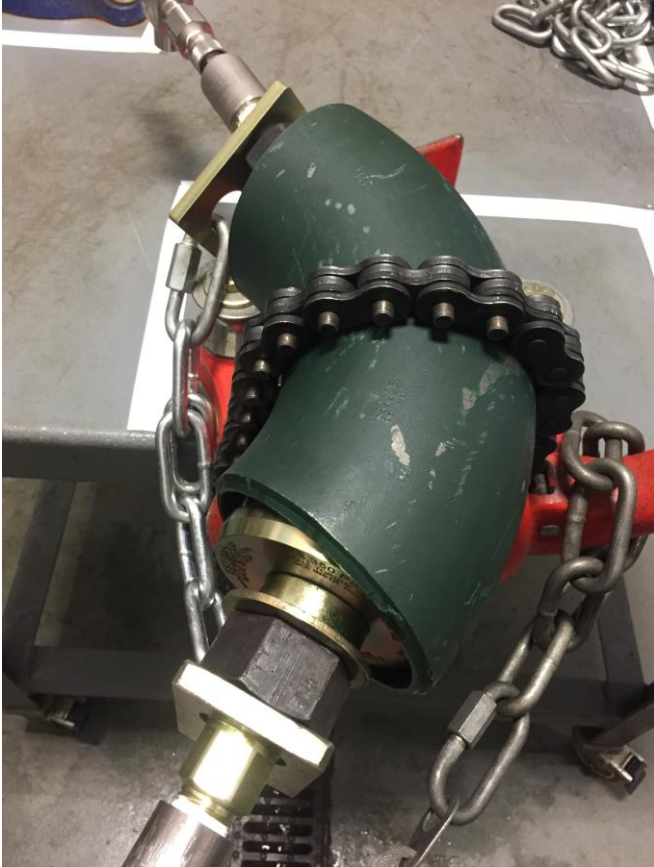
Test setup on 4" and 8" sch. 40 elbow:
